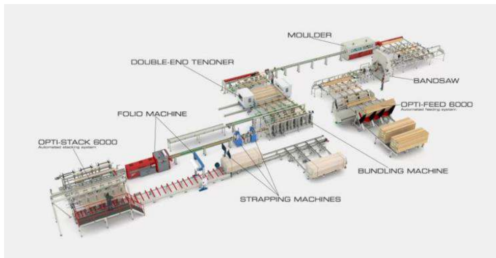
Рис. 4. Opti-Solution
